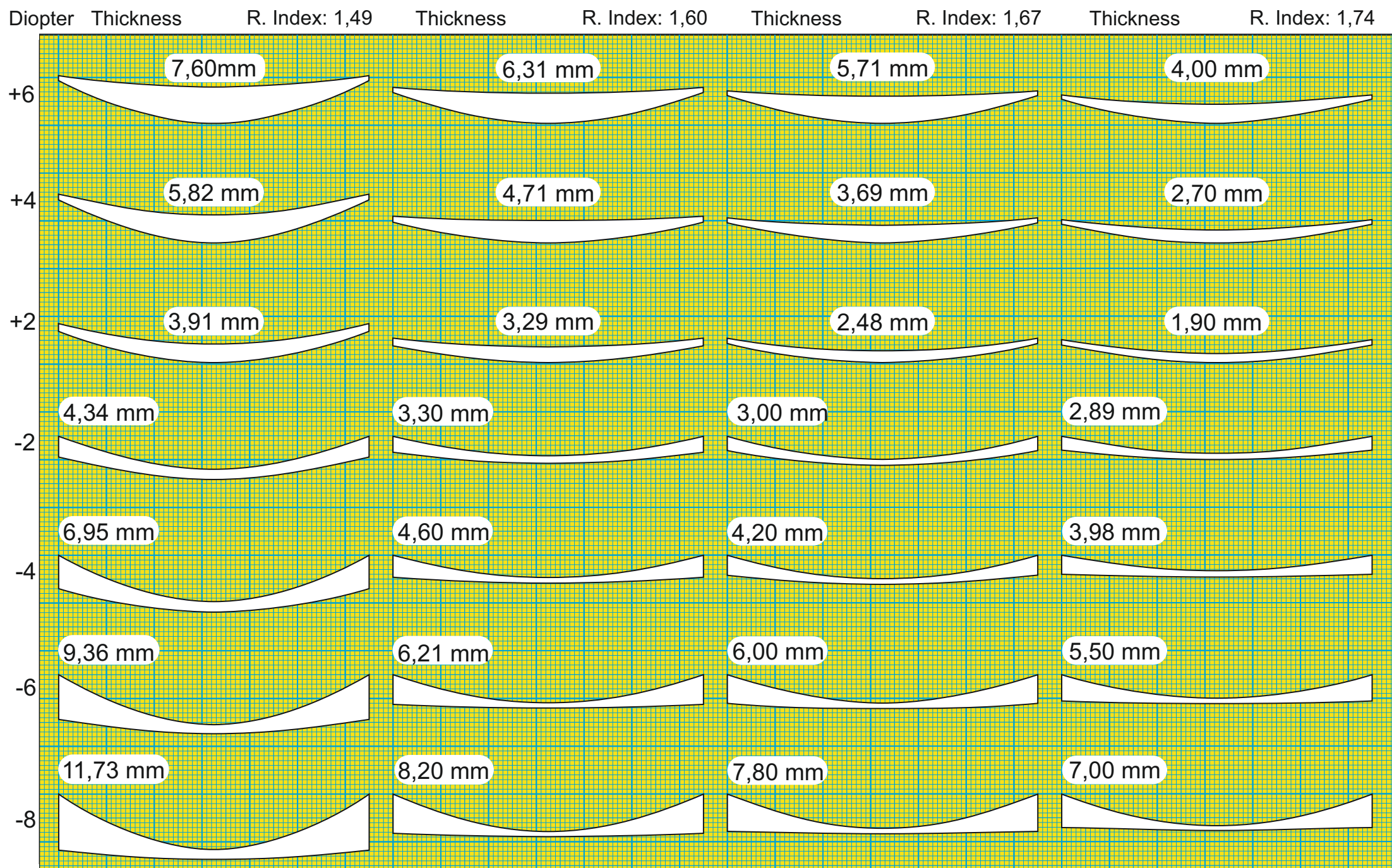
Figure: Schematic drawing showing the thinning of optical lenses with different raw material refractive indices for various diopters. This is a guide only; lens shape may vary depending on prescription and frame selection. Inspired by a different lens manufacturer's catalog, drawn by Dr. Ercan Mensiz. Freely distributable. www.amansees.com
